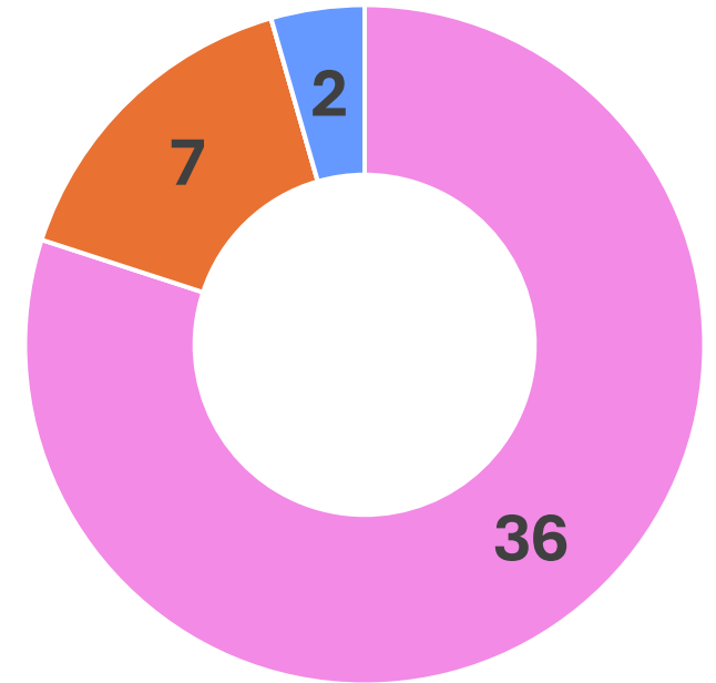
Chemistry
